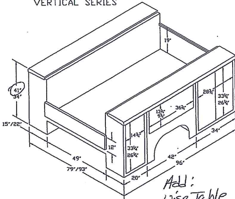
STANDARD OPEN-TOP VERTICAL SERIES
