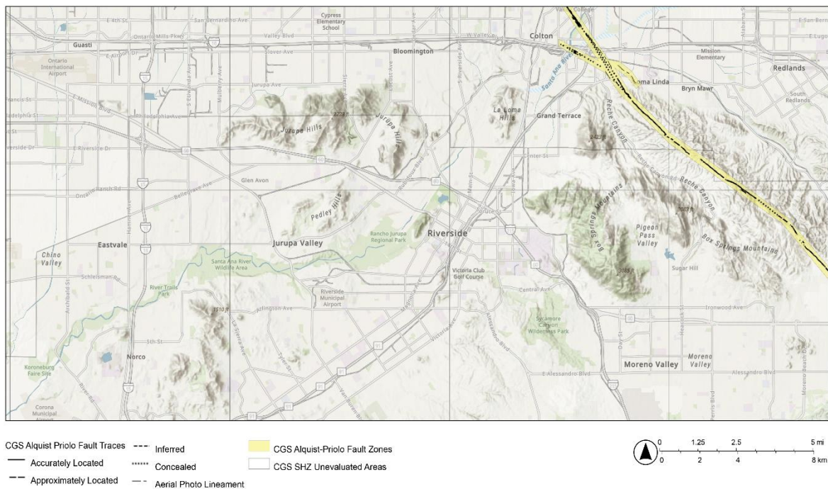
Figure 5.3: Seismic Hazards within RCSD's Service Area (California Geological Survey)
