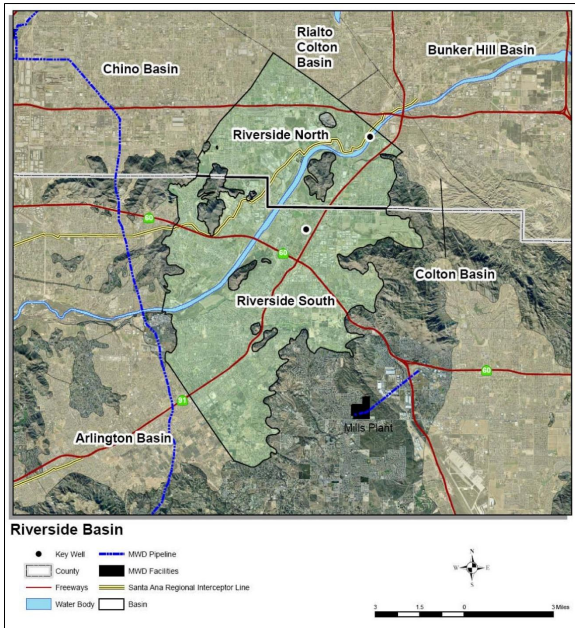
Figure 3.1: Local Groundwater Basins
