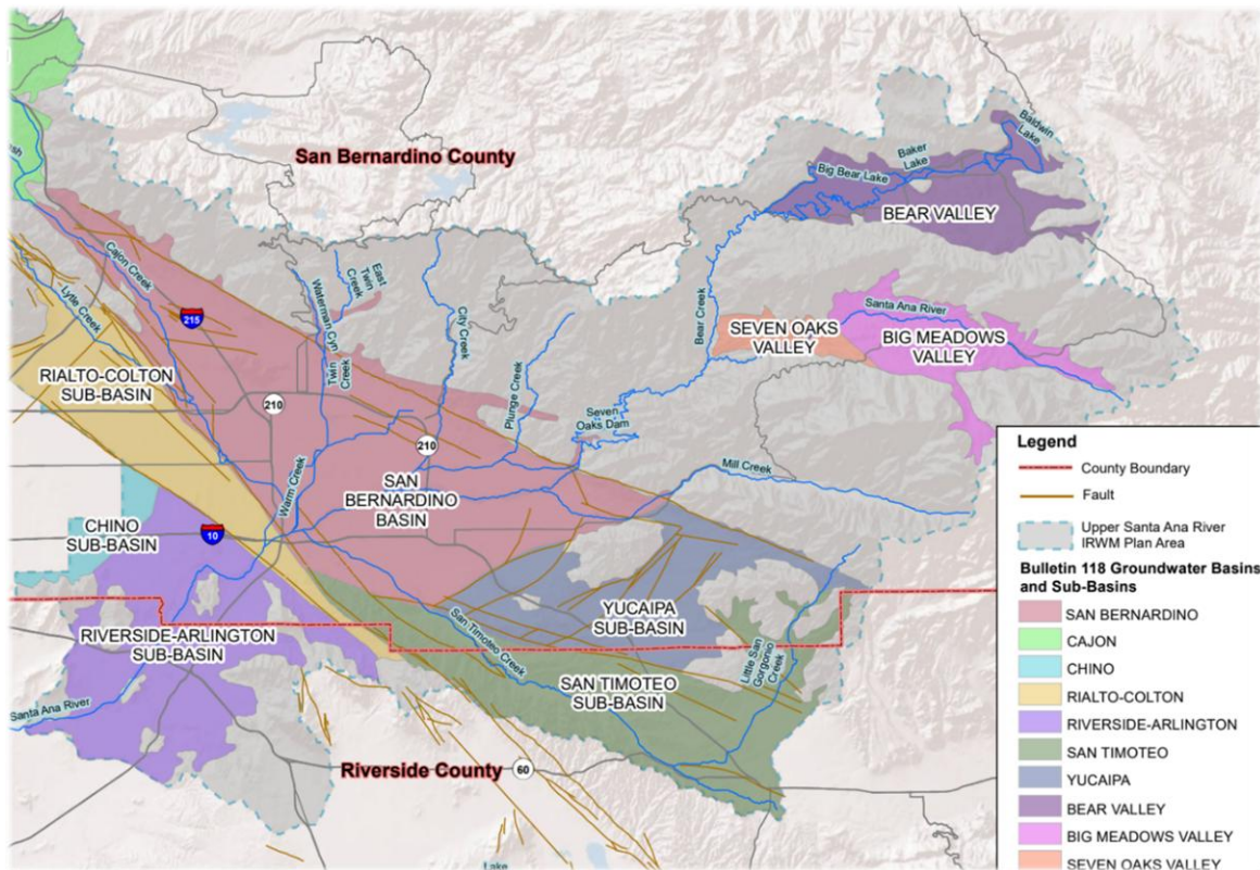
Figure 3.2: Riverside-Arlington Subbasin (Solid Purple, Lower Left)
